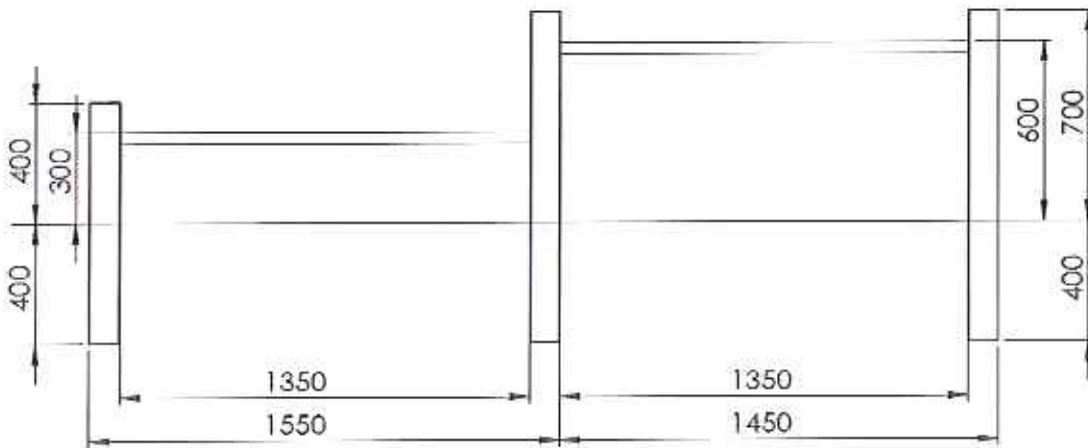
VISTA FRONTAL
